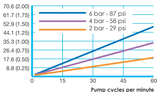
Motor air consumption (m 3 /min.) (Cubic feet/min).
